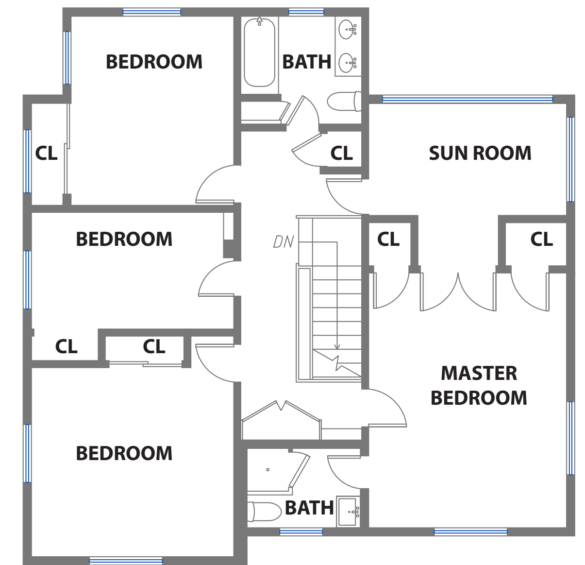
UPPER LEVEL
